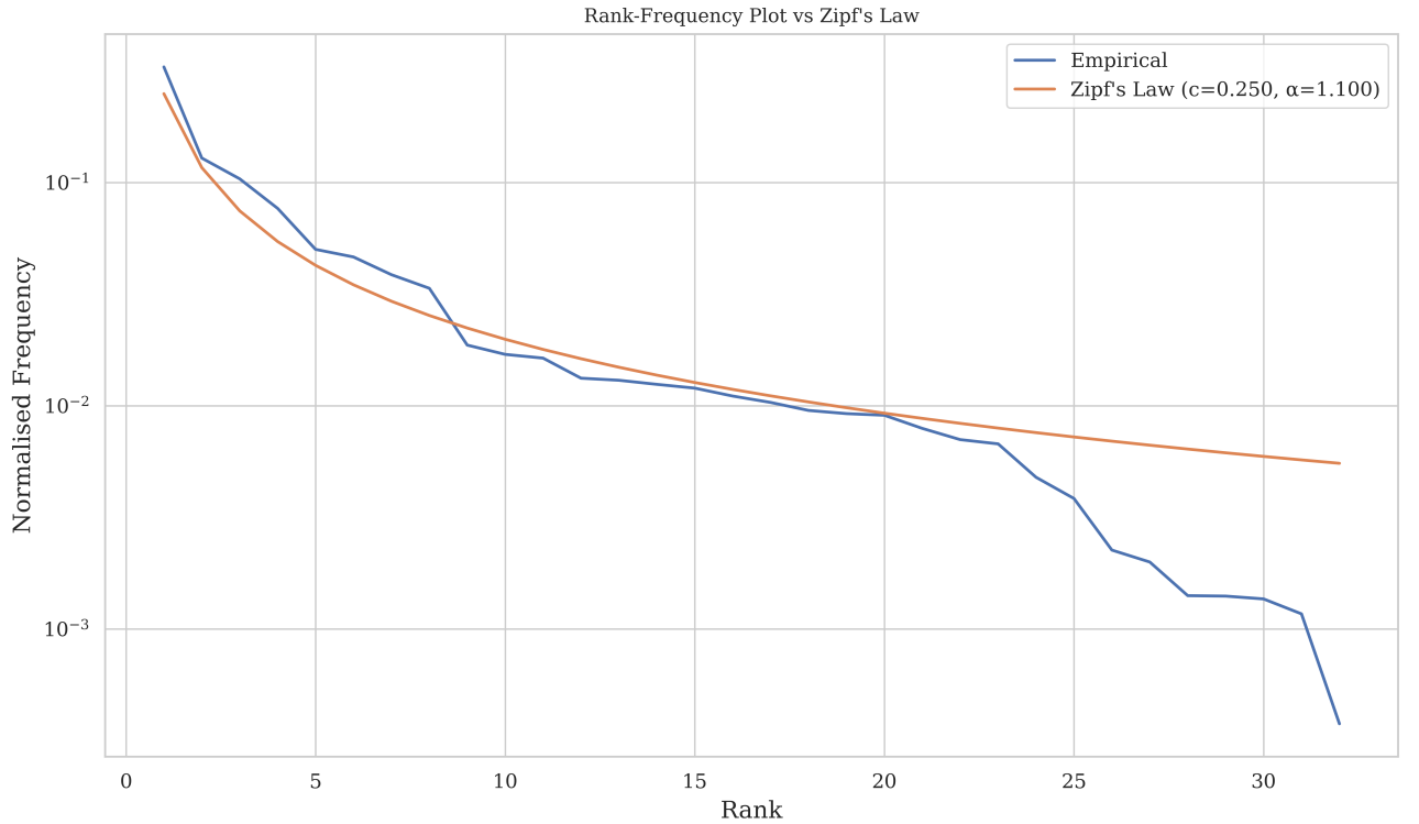
Figure 4.6: Vocabulary rank-frequency plot compared to Zipf’s Law.
