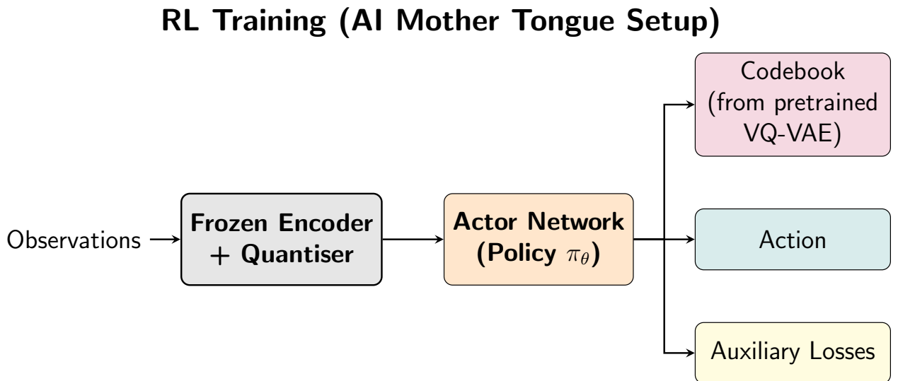
Figure 2.2: Diagram of the AI Mother Tongue architecture as proposed by Liu.
